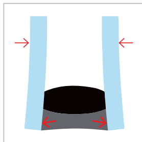
Contracted IGU
