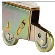
Corrosive-resistant, heavy-duty, ball-bearing 1-1/4" dual wheel keeps your door reliably on track.
